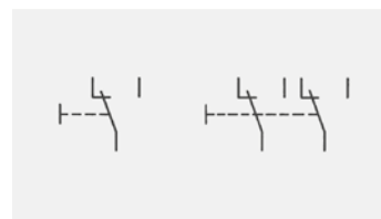
Wechsler / Taster (SPDT Momentary, DPDT Momentary)
