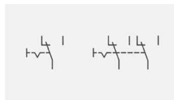
Changeover switch (SPDT)
