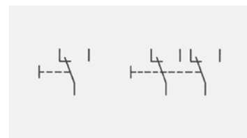
Changeover switch / pushbutton (SPDT momentary, DPDT momentary)
